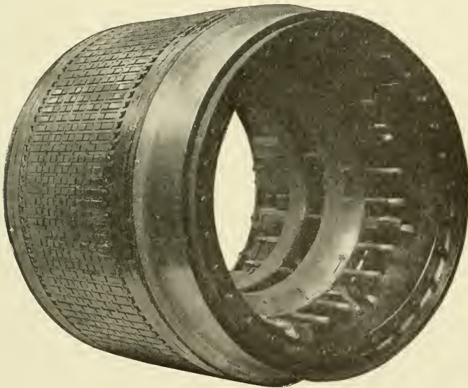
Fig. 253. Armature and Commutator of Pennsylvania Motor
